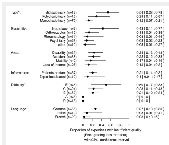
Figure 3 Influence of studied factors on the rating of overall quality. Factors that had a significant influence (type, difficulty, and language) are marked with a star. The number of expertises (n) in each category is indicated as well as the estimate and its 95% confidence interval.
